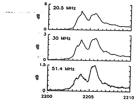
Figure 79 - Absorption records from broad-beam riometers.
