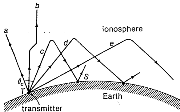
Figure 4 - A ray diagram for HF waves penetrating the ionosphere while MF waves are refracted back to earth on hops.
