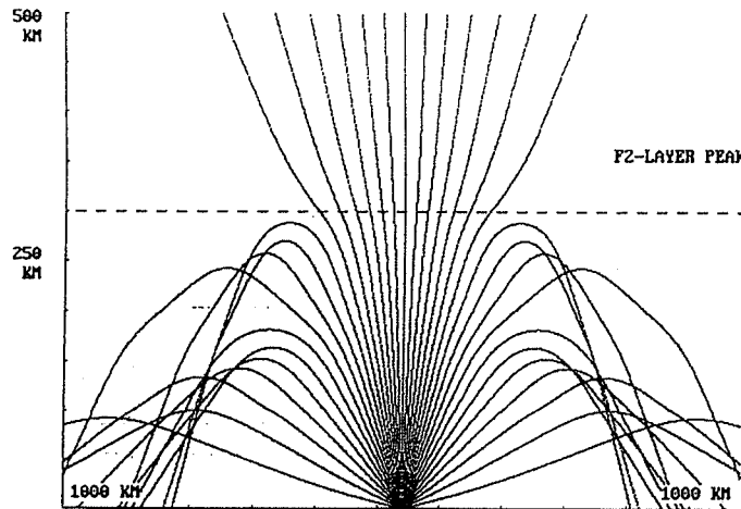
Figure 42 - Ray-tracing for 7.0 MHz with an "iris" of rays penetrating the F-peak, 5-90 degs in 5 deg steps.
