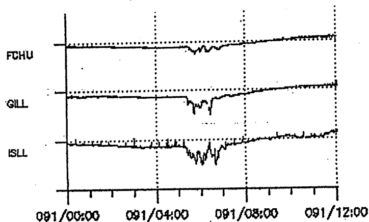
Figure 77 - Absorption records along a N-S riometer chain.
