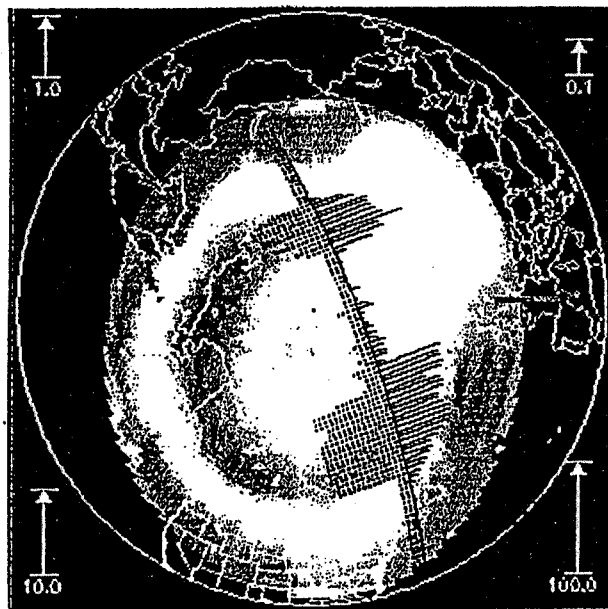
Figure 91 - NOAA 14 satellite pass across the northern polar cap.
